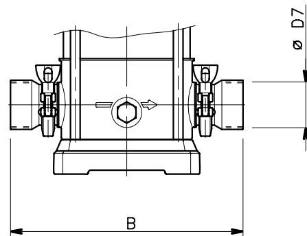
THREADED SLEEVES
